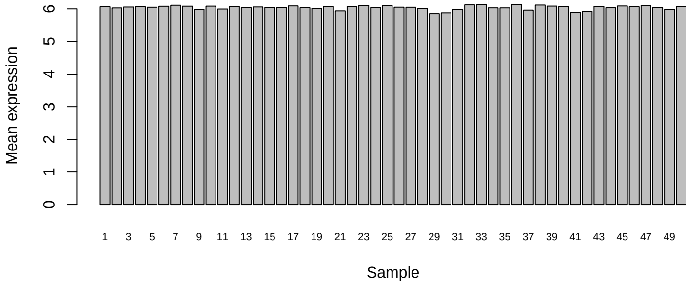
Mean expression across samples
